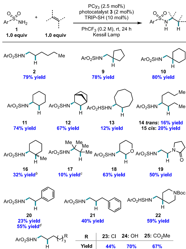
Figure 4. Olefin scope. a Reactions performed on a 0.5 mmol scale with 1.0 equiv of sulfonamide 1 (Ar = p - tert -butylbenzene) and 1.0 equiv of olefin. Isolated yield, reported as an average of two runs. b 1:2 cis/trans mixture of diastereomers. c Reaction was conducted with 3.0 equiv of olefin. d 1 H NMR yield determined by comparison to an internal standard.
