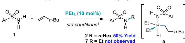
Figure 3. Mechanistic studies. a Standard conditions: as in entry 16, Table 1 without PCy 3 .
