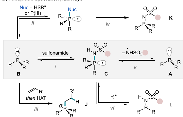
Figure 2. Proposed catalytic cycle and alternative speciation pathways.
