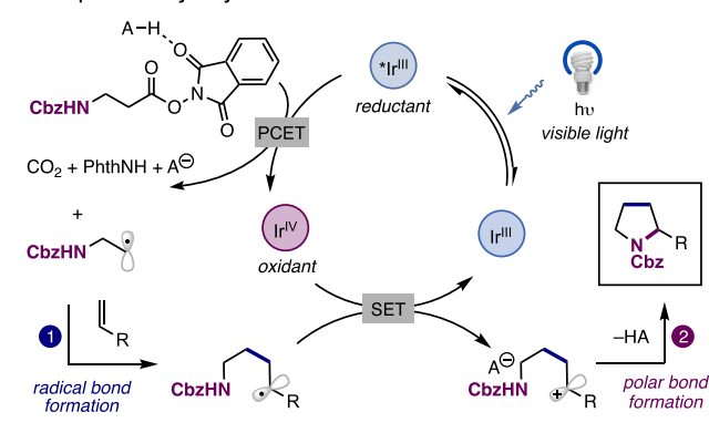
Figure 1. (A) Examples of classic annulation reactions in chemical synthesis. (B) Recent related catalytic methods for two-component annulation. (C) This work: a photocatalytic, two-component annulation of redox-active phthalimides and alkenes. (D) Proposed catalytic cycle.
